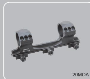
30mm One Piece Medium Picatinny Mount XASR-3010 / XASR-3011 | Center Height 1.25" (32mm)
