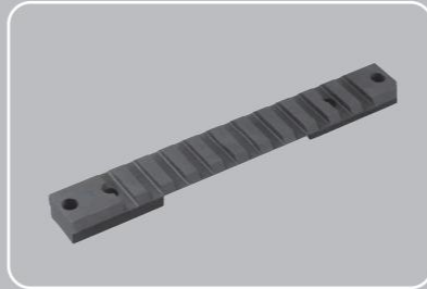
138mm / 5.4" R700 Steel Rail Short | SCRA-64
